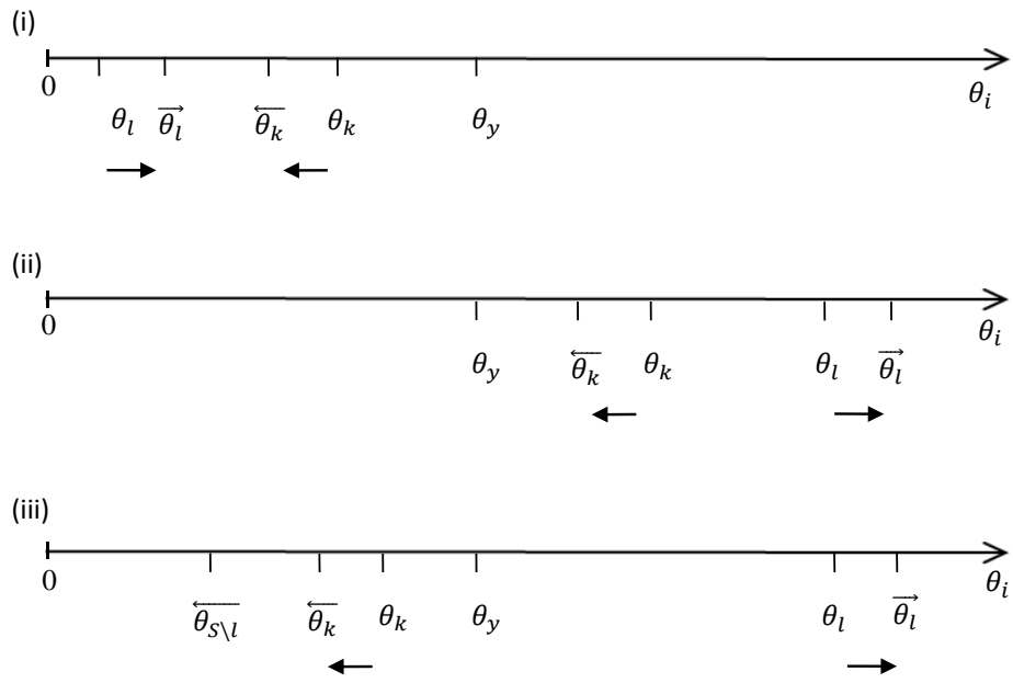
Figure 2: Illustration of Proposition 2
